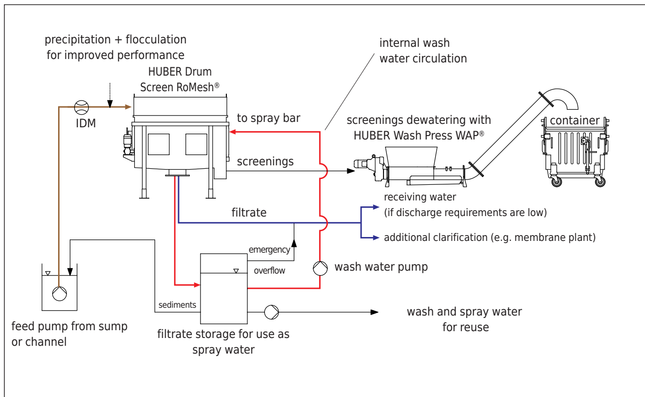
Flow diagram of mechanical wastewater treatment with a HUBER Drum Screen RoMesh®
