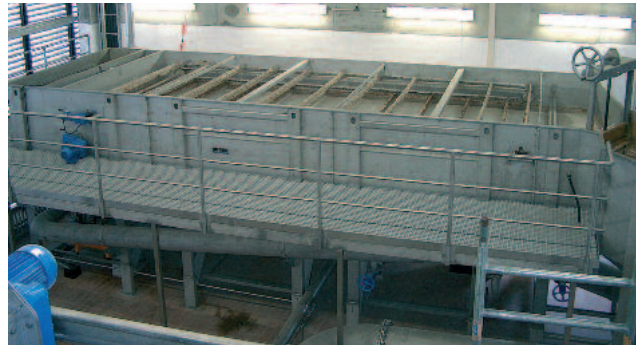
HUBER Dissolved Air Flotation Plant HDF without chemical treatment stage for up to 400 m 3 /h
