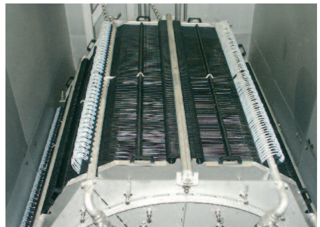
HUBER Vacuum Rotation Membrane VRM® Bioreactor
