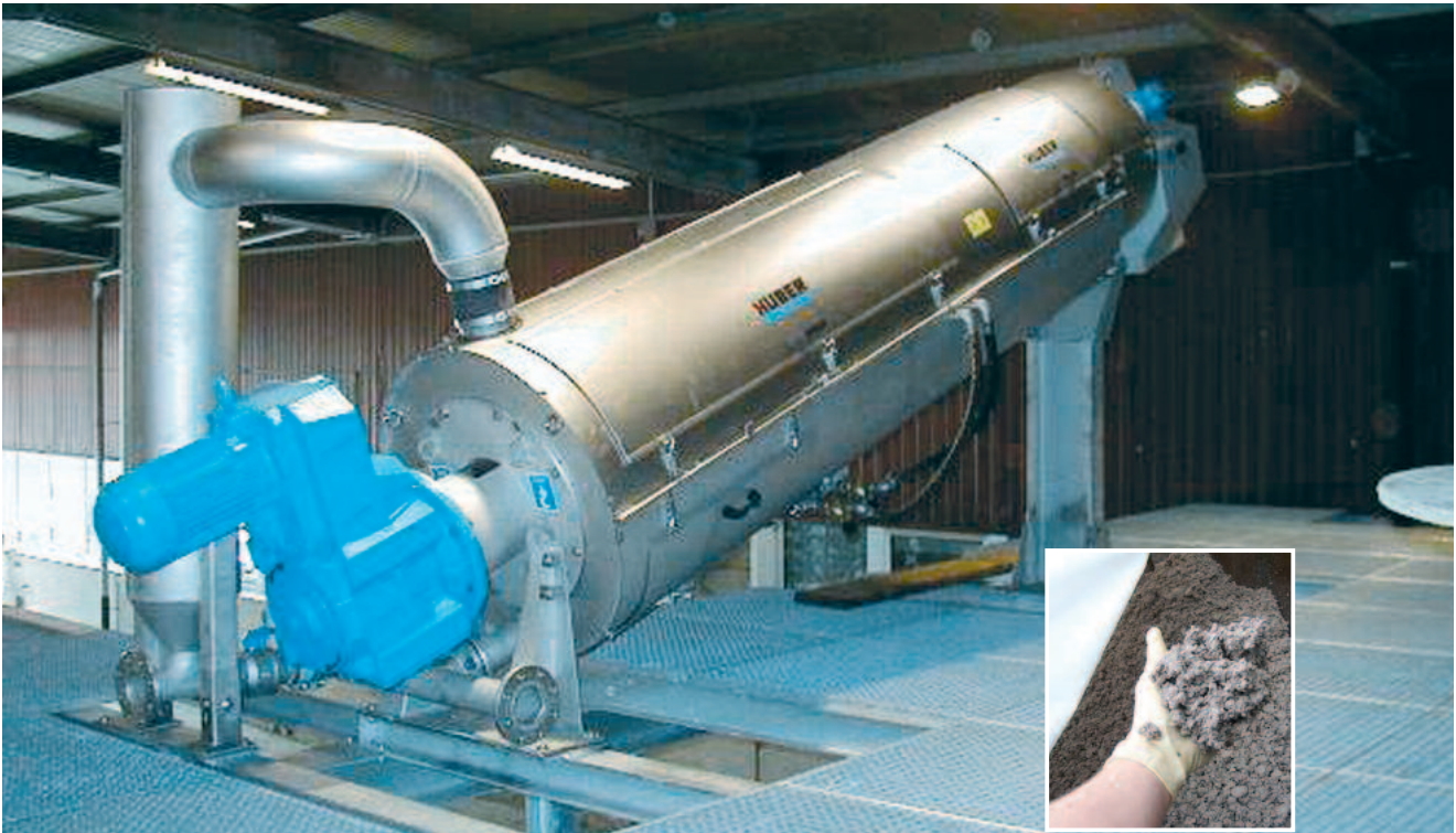
Flotate sludge dewatering with HUBER ROTAMAT® Screw Press RoS 3 Image detail: Dewatered flotate sludge with > 30 % DS content
