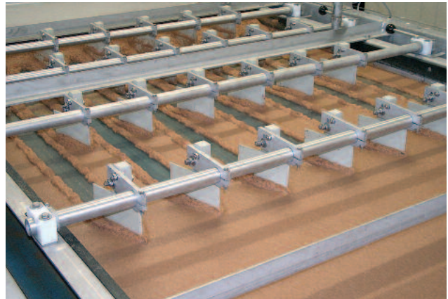
HUBER Drainbelt – Uncomplicated, efficient biological sludge thickening
